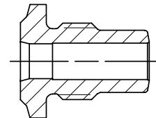
126302 DRIVING ANVIL -08
