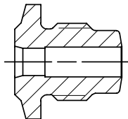
126301 DRIVING ANVIL -06
