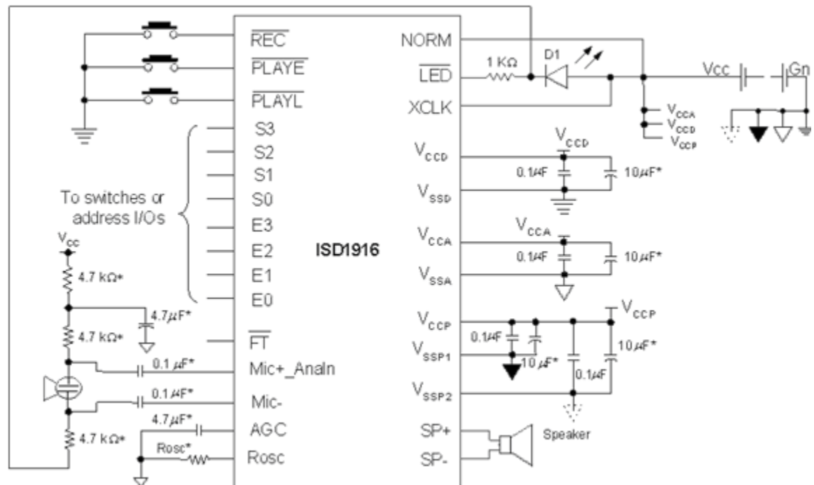
Application Diagram
