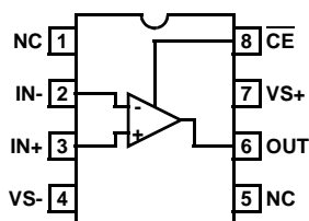
EL5132 (8 LD SOIC) TOP VIEW
