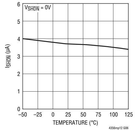
I_{SHDN} Current vs Temperature
