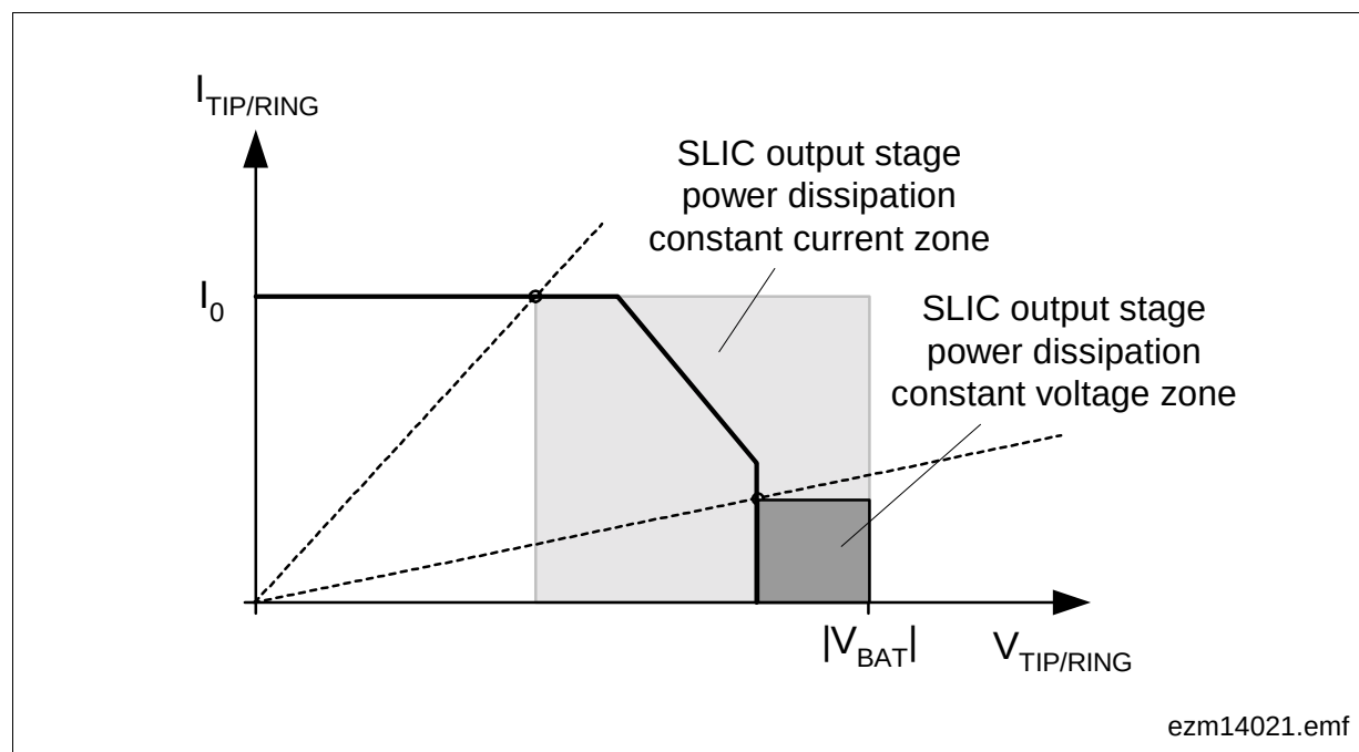
Figure 19 Power Dissipation
