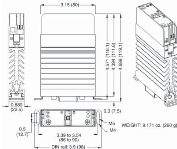
Figure 1 — DRS relay; dimensions in inches (mm)
