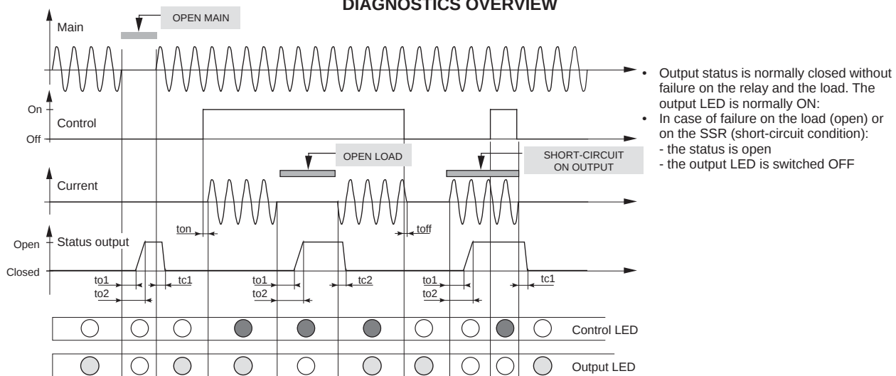
Figure 8 — DRS relay
