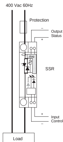
Figure 2 — DRS relay (See Note 4)
