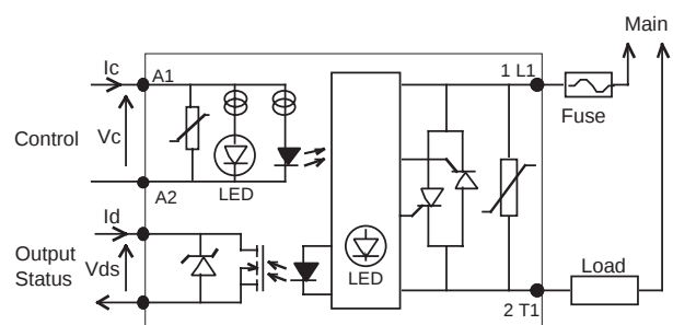
Figure 4 — DRS relay
