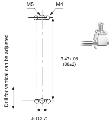
Figure 10 — DRS relay
