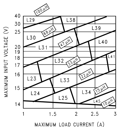
Figure 23. LM2670-12
