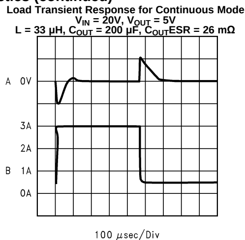
A: Output Voltage, 100 mV/div, AC-Coupled B: Load Current: 500 mA to 3A Load Pulse Figure 17.
