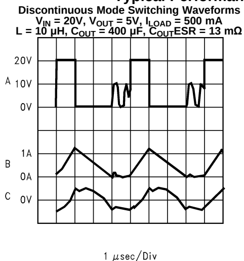
A: V_{SW} Pin Voltage, 10 V/div B: Inductor Current, 1 A/div C: Output Ripple Voltage, 20 mV/div AC-Coupled Figure 16.
