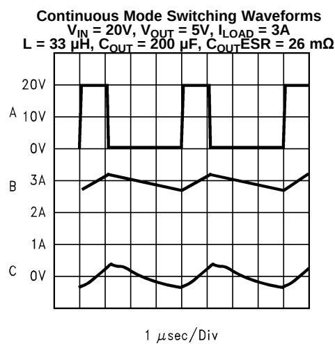
A: V_{SW} Pin Voltage, 10 V/div B: Inductor Current, 1 A/div C: Output Ripple Voltage, 20 mV/div AC-Coupled Figure 15.
