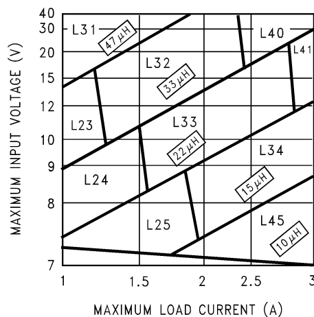
Figure 22. LM2670-5.0
