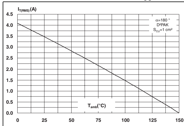
Figure 3. RMS on-state current vs ambient temperature, PCB FR4, e_{CU} = 35 \mu m
