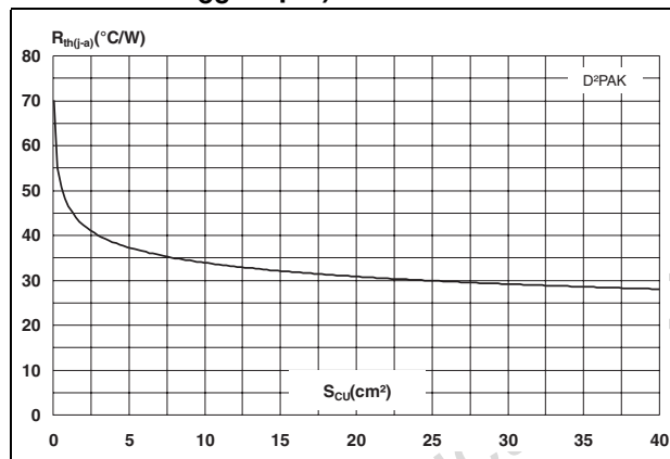
Figure 11. Variation of thermal resistance, junction to ambient versus copper surface under tab (PCB FR4, e_{Cu} 35 μm)
