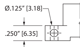
FLUSH MOUNTING WITH SIDE HOLES (Z)
