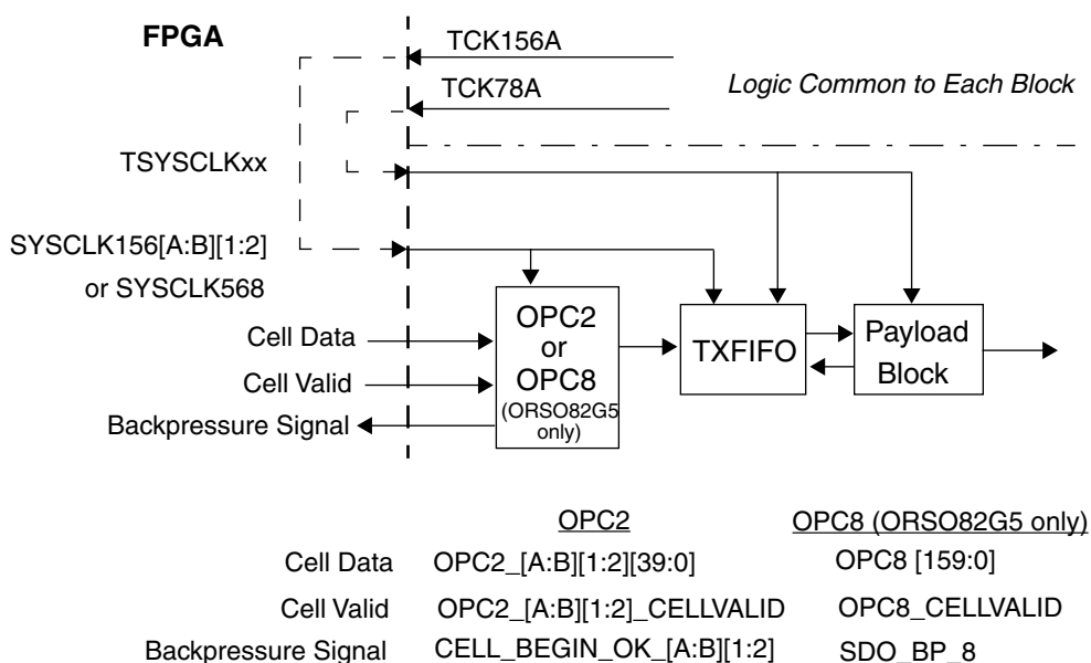
Figure 40. Cell Mode Transmit Timing
