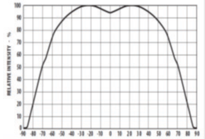
Figure 4 Radiation Pattern
