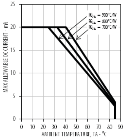
Figure 7 Derating Curve
