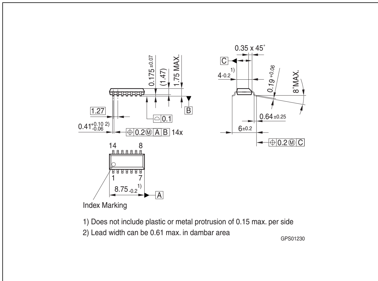
Figure 7 PG-DSO-14-30 (Plastic Dual Small Outline)
