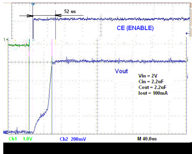
Figure 26. Turn On Speed NCP693xMN08CTG
