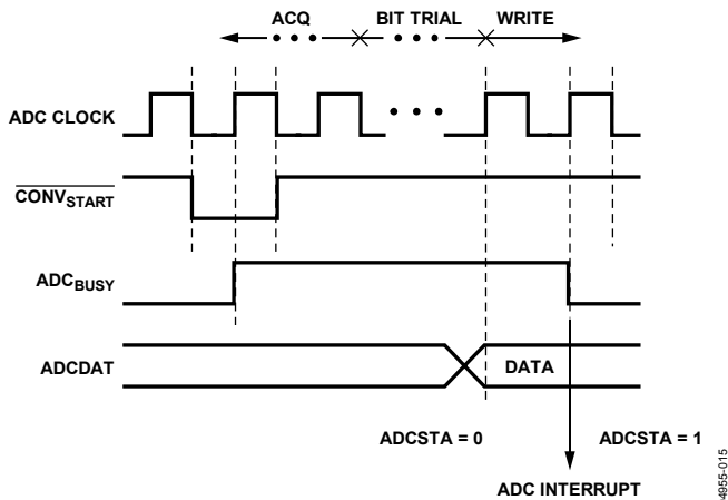
Figure 41. ADC Timing
