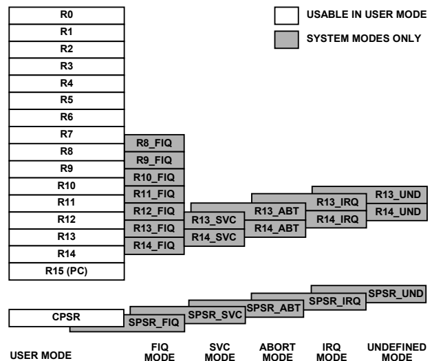
Figure 33. Register Organization
