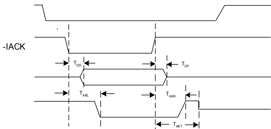
Figure 7: Interrupt Timing
