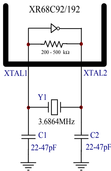
Figure 1: Crystal Connection
