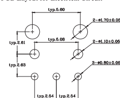
PCB Layout for Electrical Circuit
