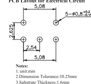
PCB Layout for Electrical Circuit
