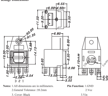
Package Dimensions
