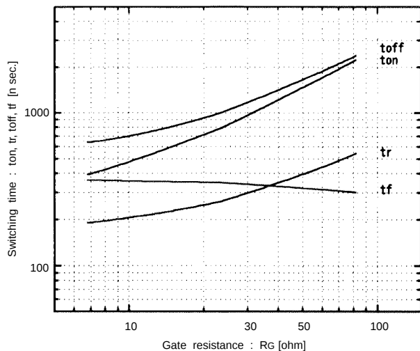
Switching time vs. R_G V_{CC}=600V , I_C=75A , V_{GE}=\pm 15V , T_J=25^\circ C
