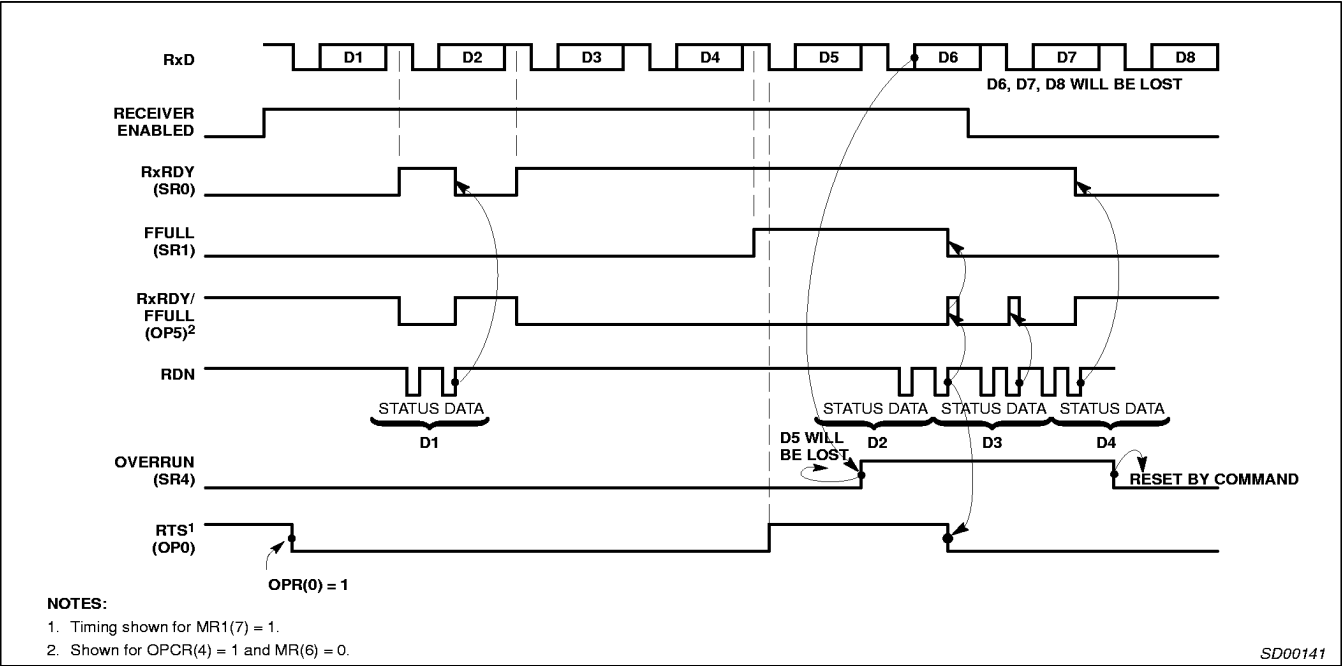
Figure 11. Receiver Timing
