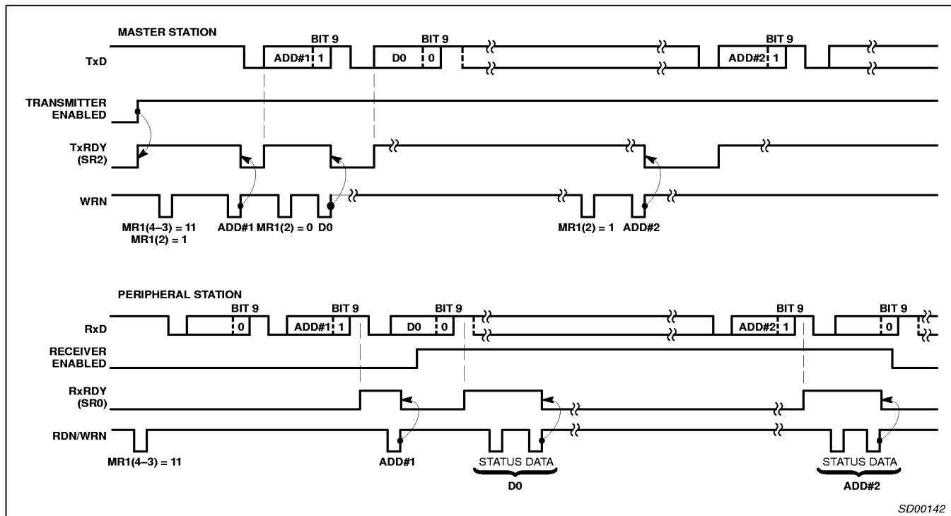
Figure 12. Wake-Up Mode
