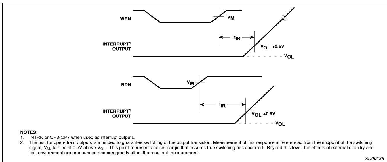
Figure 6. Interrupt Timing
