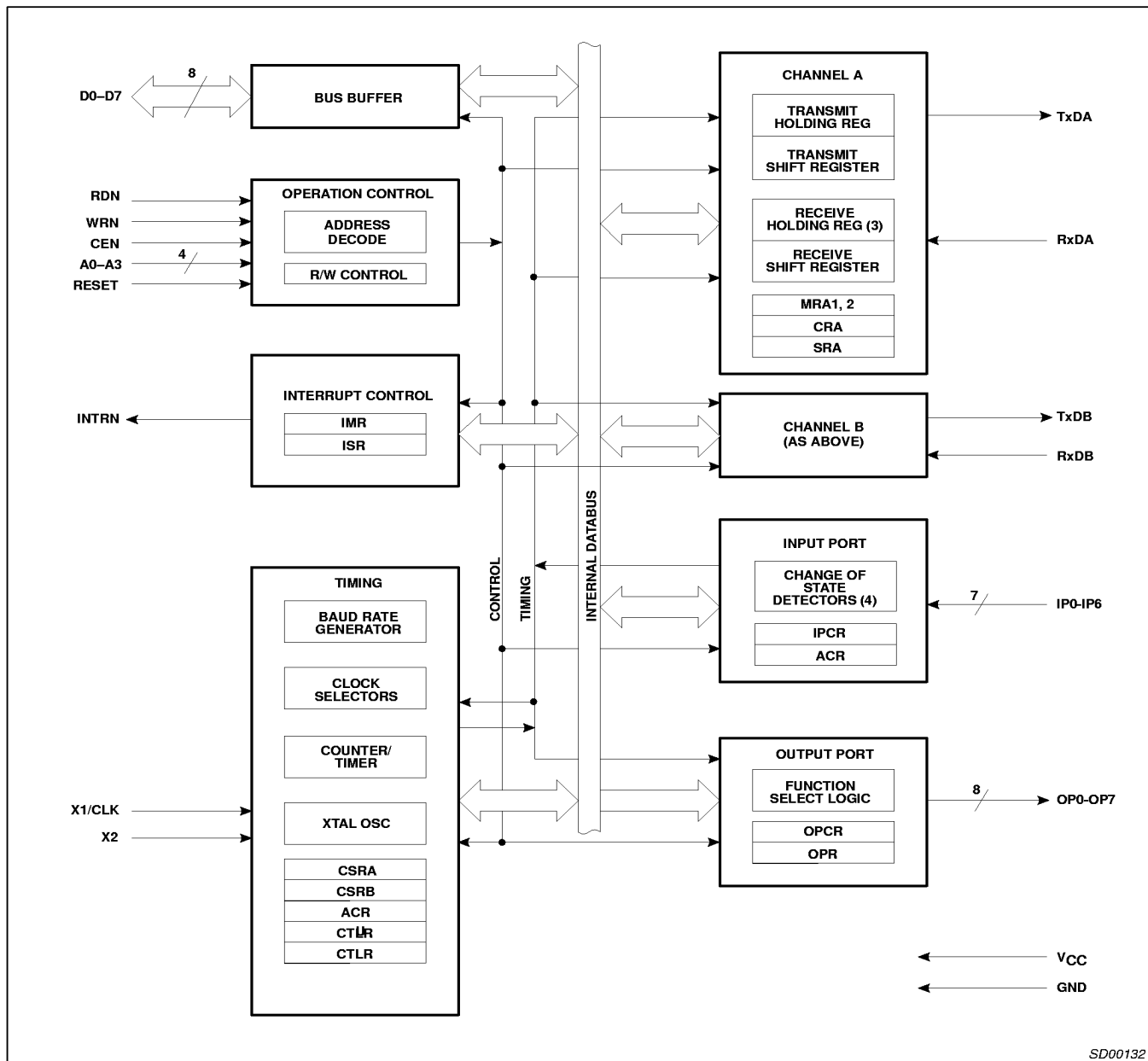
Figure 2. Block Diagram
