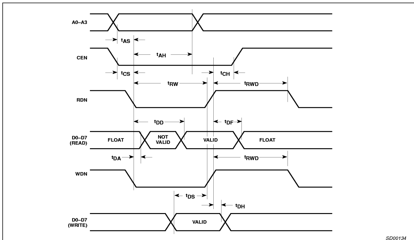
Figure 4. Bus Timing
