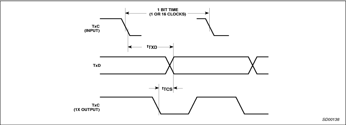
Figure 8. Transmitter External
