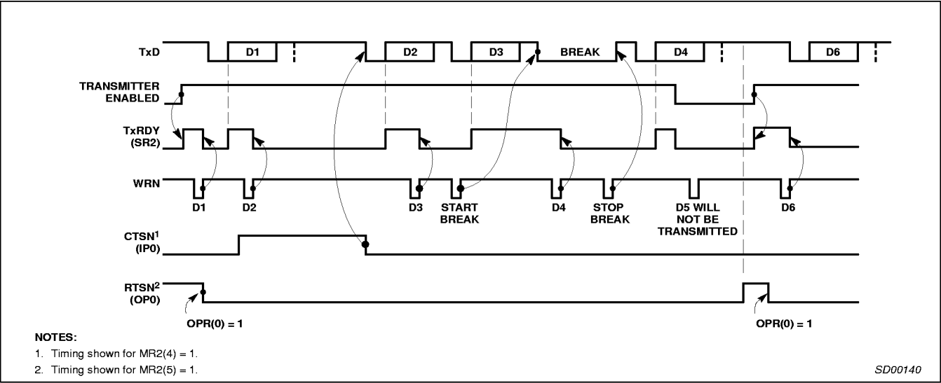
Figure 10. Transmitter Timing
