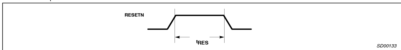
Figure 3. Reset Timing
