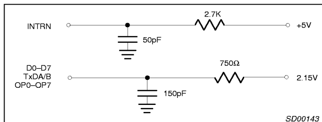
Figure 13. Test Conditions on Outputs
