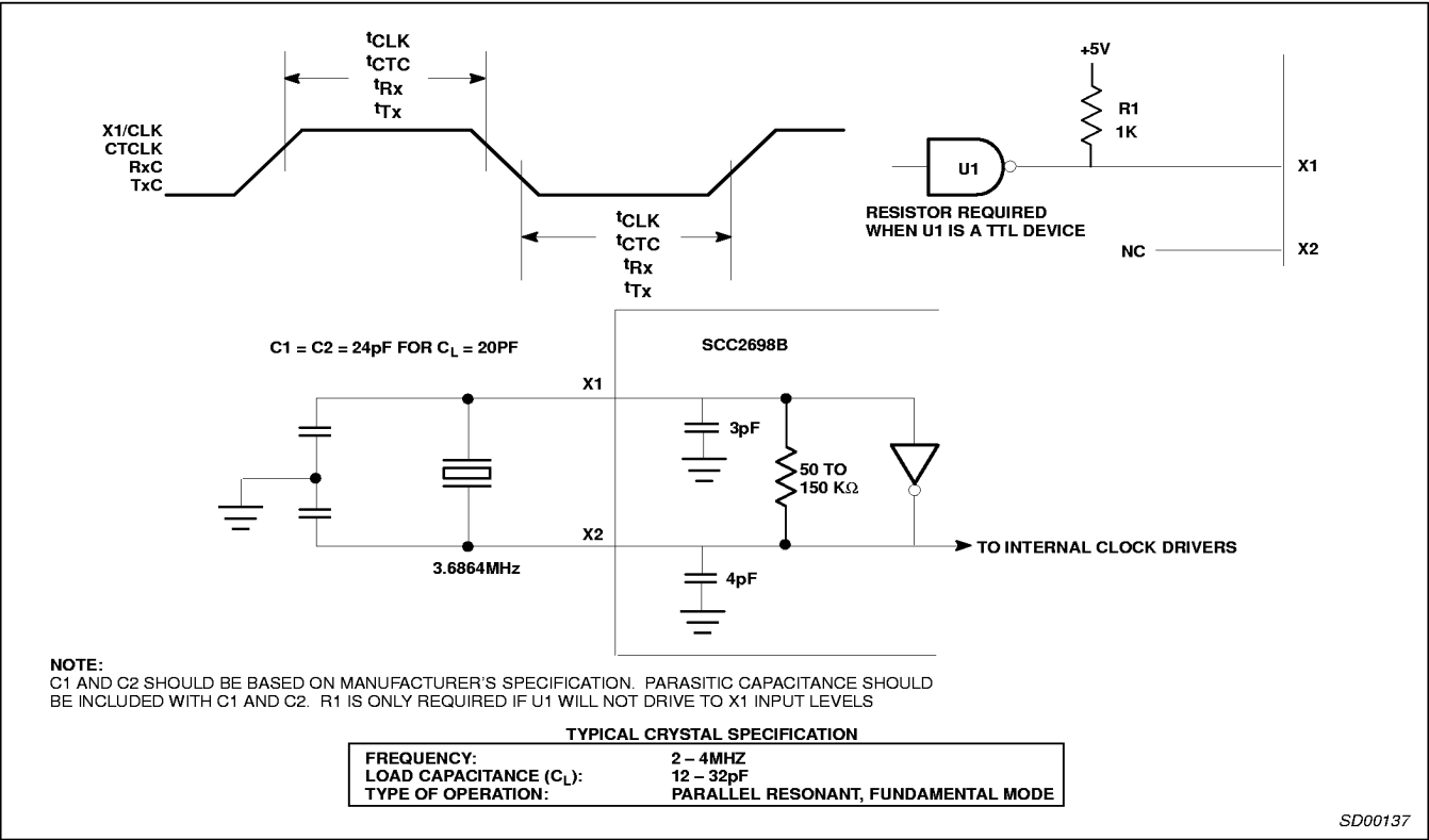
Figure 7. Clock Timing
