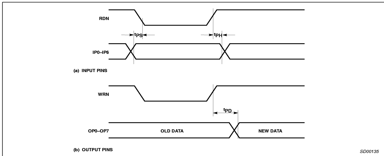
Figure 5. Port Timing
