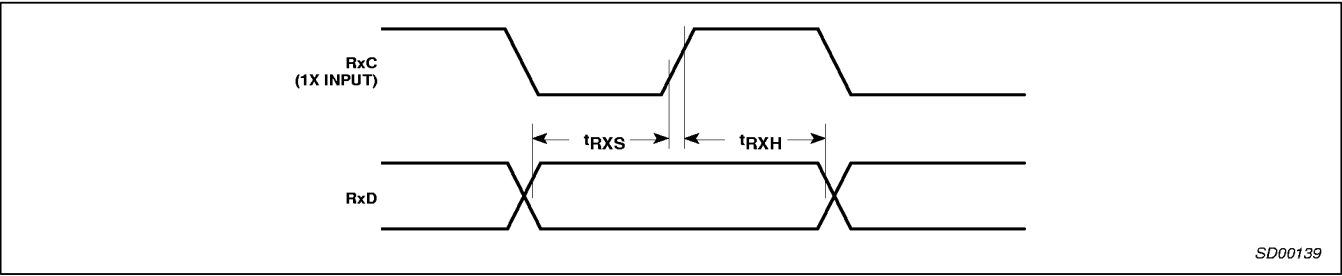
Figure 9. Receive External Clock
