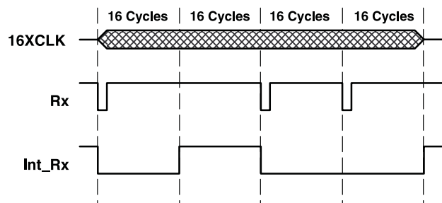
Figure 31. IrDA-SIR Decoding Scheme – Macro View
