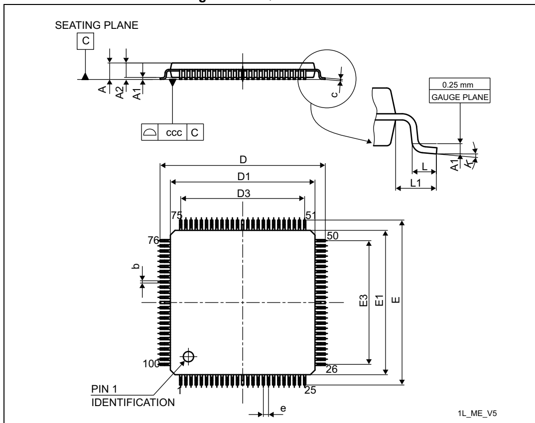
Figure 81. LQFP100 outline
