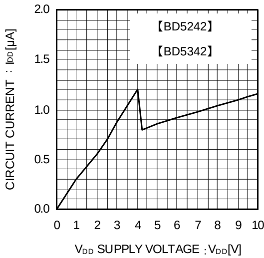
Fig.3 Circuit Current
