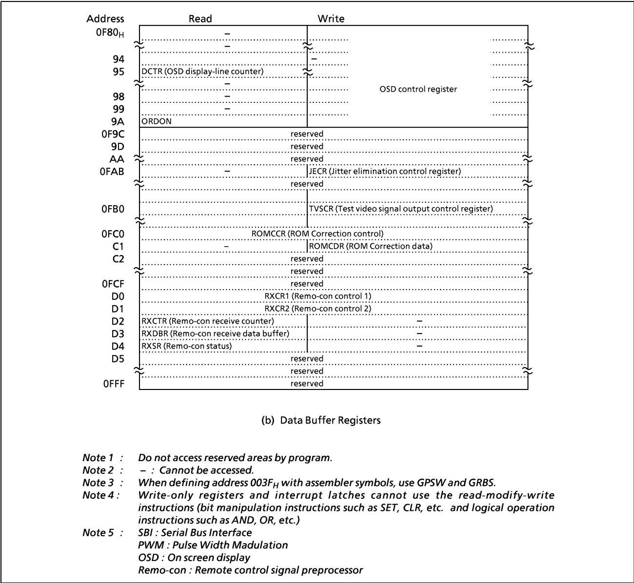
Figure 2-1-2. DBR
