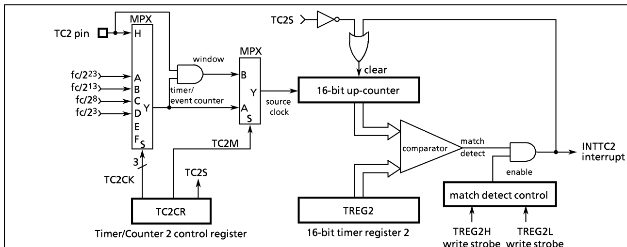
Figure 2-19. Timer/counter 2 (TC2)
