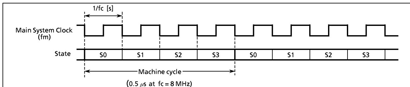
Figure 1-13. Machine cycle
