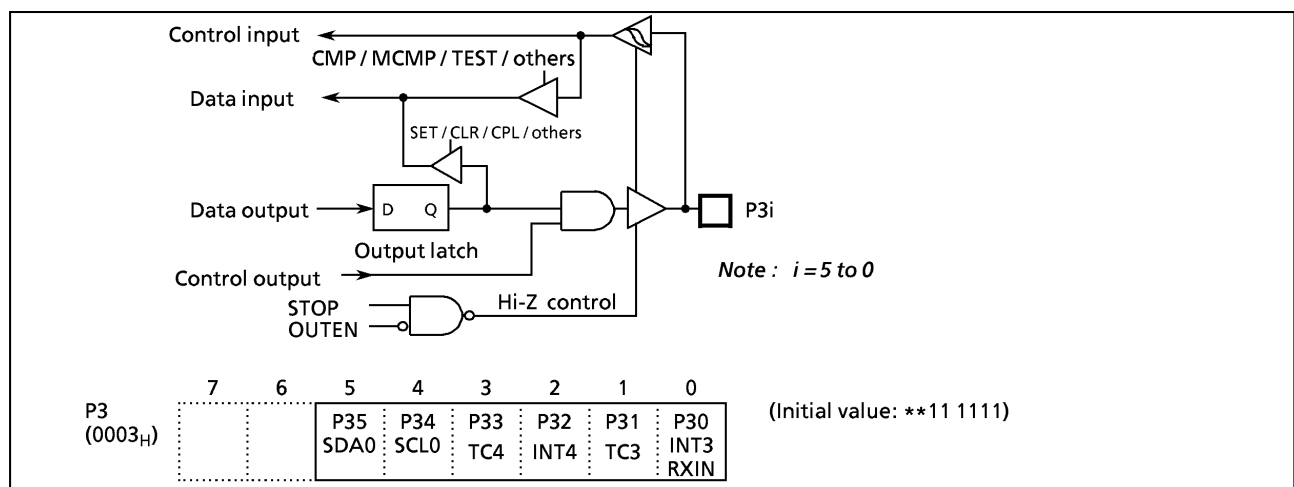
Figure 2-4. Port P3
