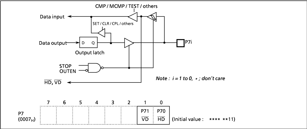
Figure 2-8. Ports P7
