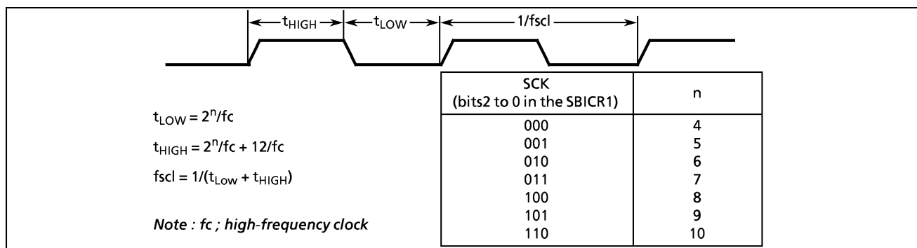
Figure 2-31. Clock source
