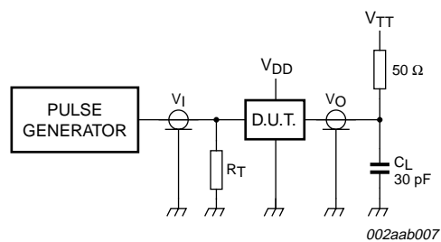
Fig 11. Load circuit for B outputs
