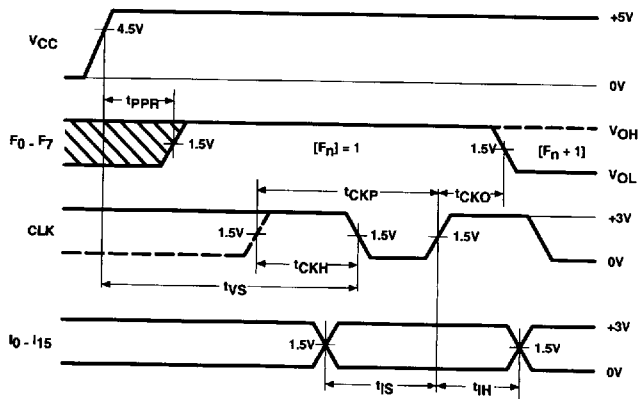
Power-On Preset
