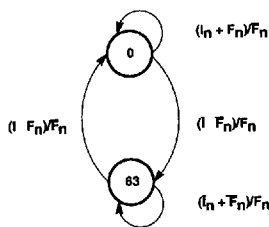
State Diagram
