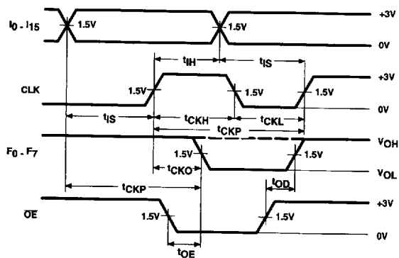
Sequential Mode
