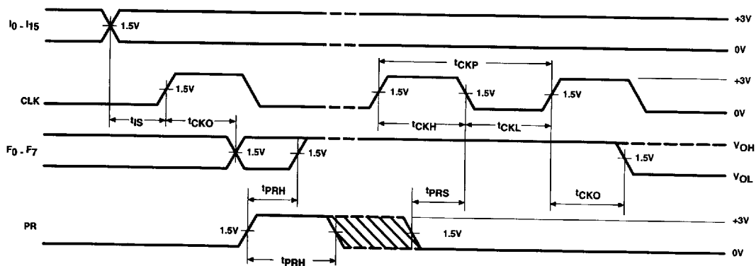
Asynchronous Preset
