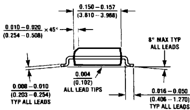
8-Pin Small Outline Package Order Number LM6142AIM or LM6142BIM NS Package Number M08A
