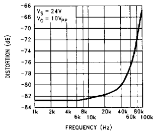
Distortion + Noise vs Frequency
