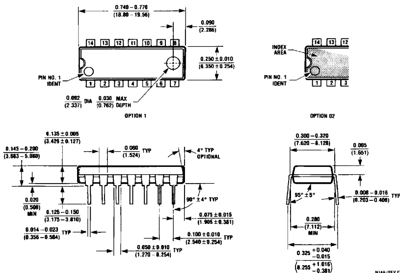
14-Pin Molded Dual-In-Line Package Order Number LM6144AIN or LM6144BIN NS Package Number N14A
