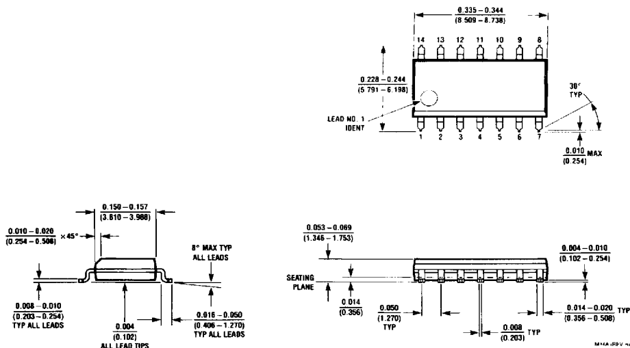
14-Pin Small Outline Package Order Number LM6144AIM or LM6144BIM NS Package Number M14A
