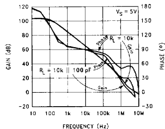
Gain and Phase vs Load
