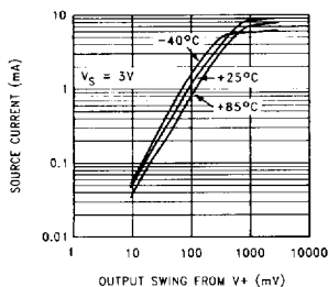
Output Voltage vs Source Current
