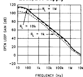
Open Loop Gain vs Load, 24V Supply
