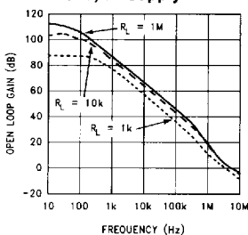
Open Loop Gain vs Load, 5V Supply
