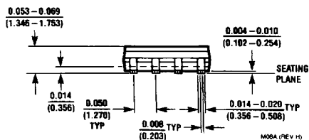
8-Pin Small Outline Package Order Number LM6142AIM or LM6142BIM NS Package Number M08A
