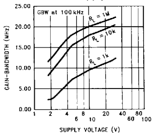
GBW vs Supply
