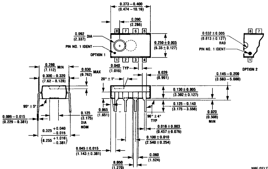
8-Pin Molded Dual-In-Line Package Order Number LM6142AIN or LM6142BIN NS Package Number N08E
