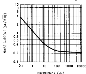
Noise Current vs Frequency
