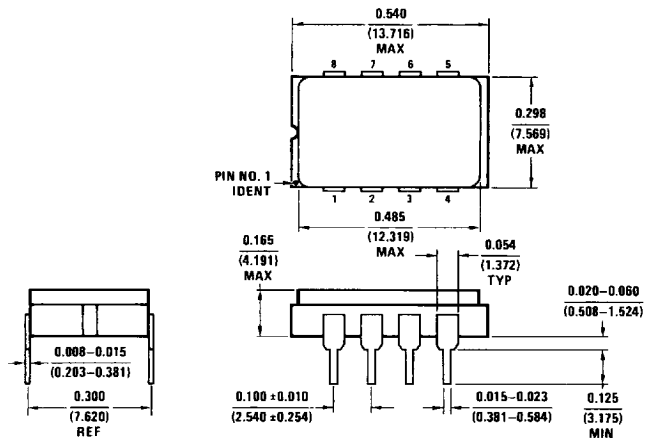
8-Pin Ceramic Sidebraced Dual-In-Line Package Order Number LM6142AMJ/883 NS Package Number D08C
