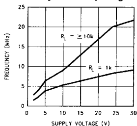
Unity Gain Freq vs V_S
