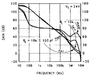
Gain and Phase vs Load
