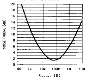
NE vs R Source
