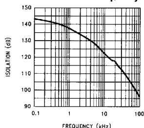
Crosstalk vs Frequency
