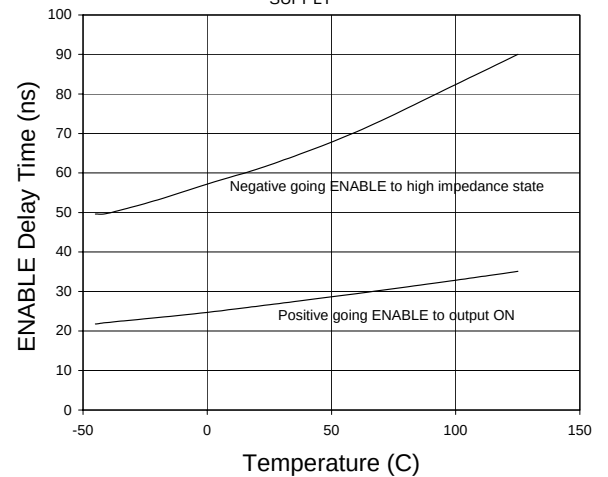
Fig. 32 ENABLE Propagation vs. Temperature V_{\text{SUPPLY}} = 15\text{V}
