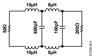
Figure 54. Fourth-Order Low-Pass W-CDMA Filter Schematic Figure 55 and Figure 56 illustrate the magnitude response and group delay response of the fourth-order filter, respectively.
