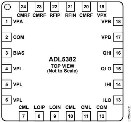
Figure 2. Pin Configuration
