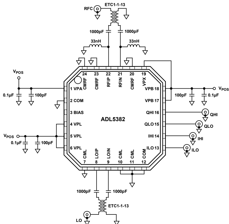
Figure 41. Basic Connections Schematic
