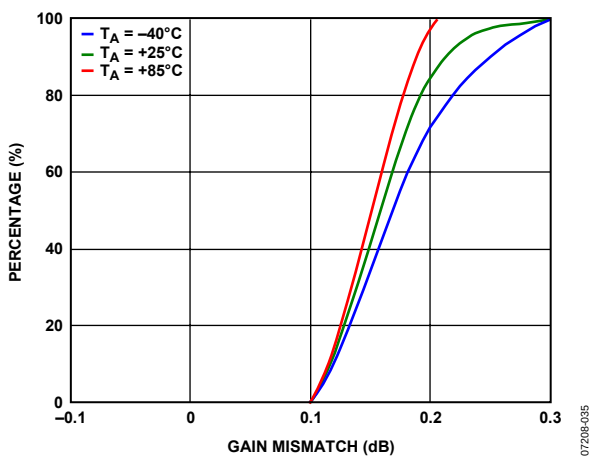
Figure 35. IQ Gain Mismatch Distributions, f_{RF} = 2700 MHz
