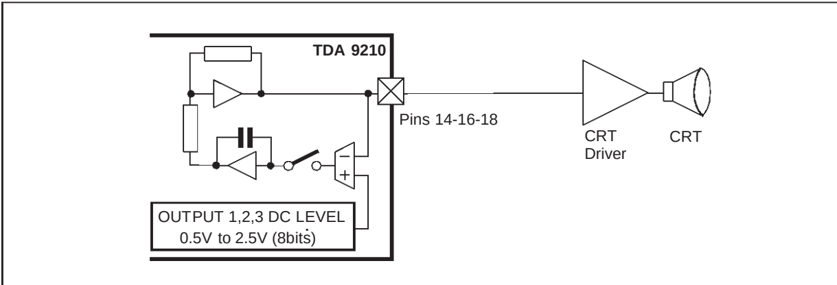
Figure 5. DC Coupling
