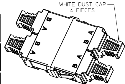
ISO VIEW 1 SCALE 1.5:1
