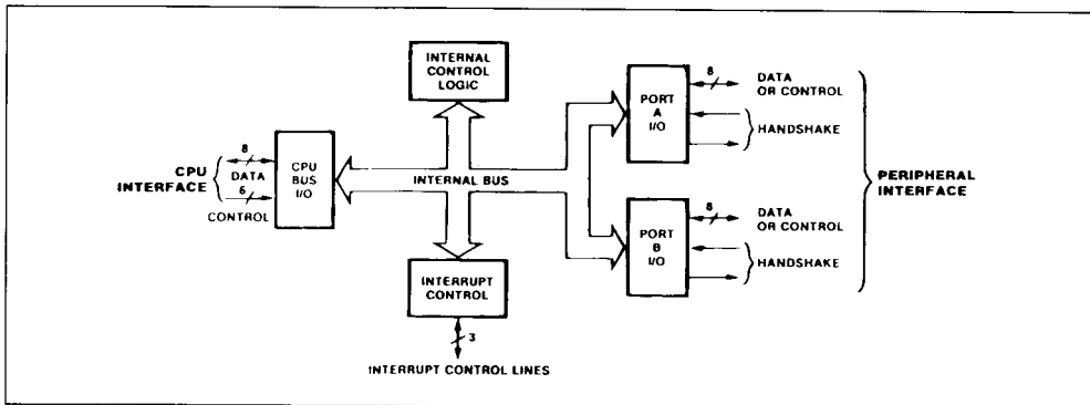
Figure 3 : Block Diagram.
