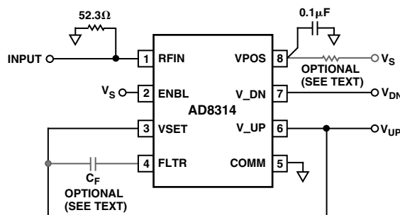
Figure 4. Basic Connections for Operation in Measurement Mode
