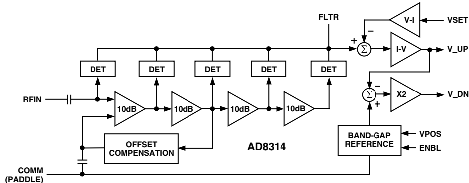
Figure 1. Block Schematic
