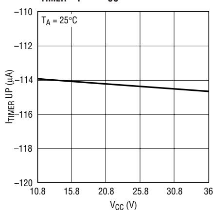
I_{TIMER} Up vs V_{CC}
