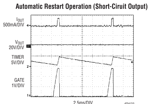
Figure 10. RETRY Waveforms
