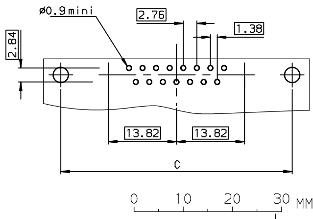
LAYOUT DIMENSIONS (after plating) CONNECTOR SIDE VIEW
