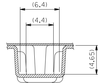
SECT. X-X
