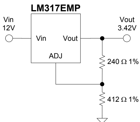
Figure 9. Suggested 3.42V Voltage Supply Circuit for SiI 1362 and SiI 1364 only
