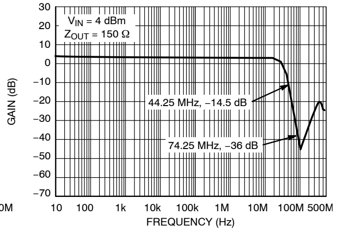
Figure 4. Attenuation
