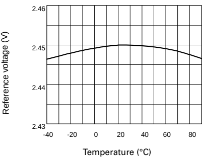
Temperature Drift
