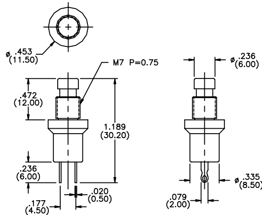
MECHANICAL OUTLINE
