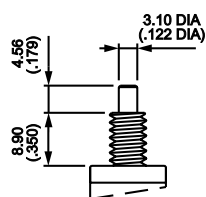
0077 Standard actuator w/threaded bushing
