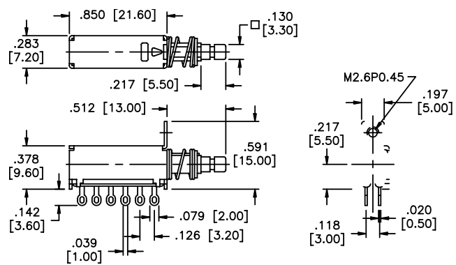
MECHANICAL OUTLINE
