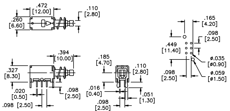
MECHANICAL OUTLINE
