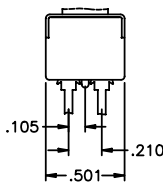
SIDE VIEW DOUBLE POLE
