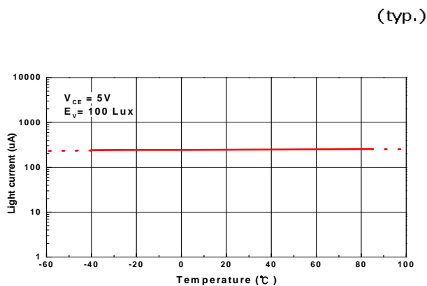
Fig.3 Light current vs. Temperature
