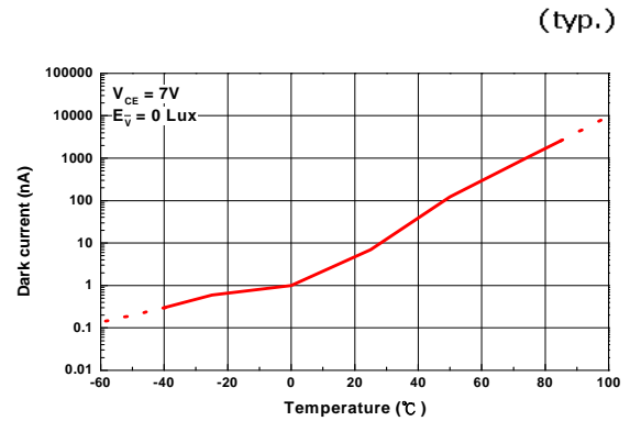
Fig.2 Dark Current vs. Temperature
