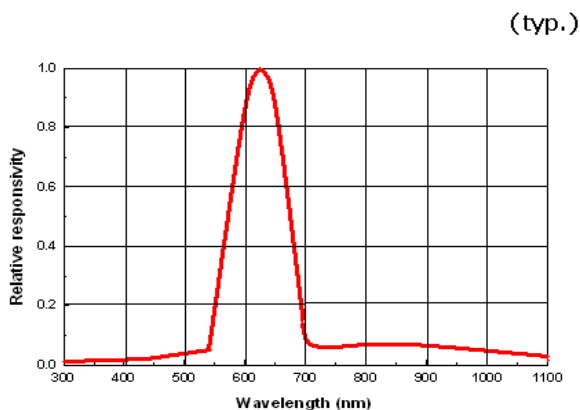
Fig.5 Spectral Response
