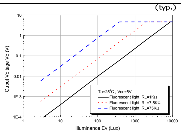
Fig.6 Output Voltage vs. Illuminance
