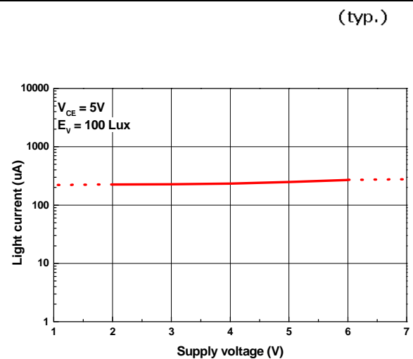
Fig.4 Light current vs. Supply Voltage
