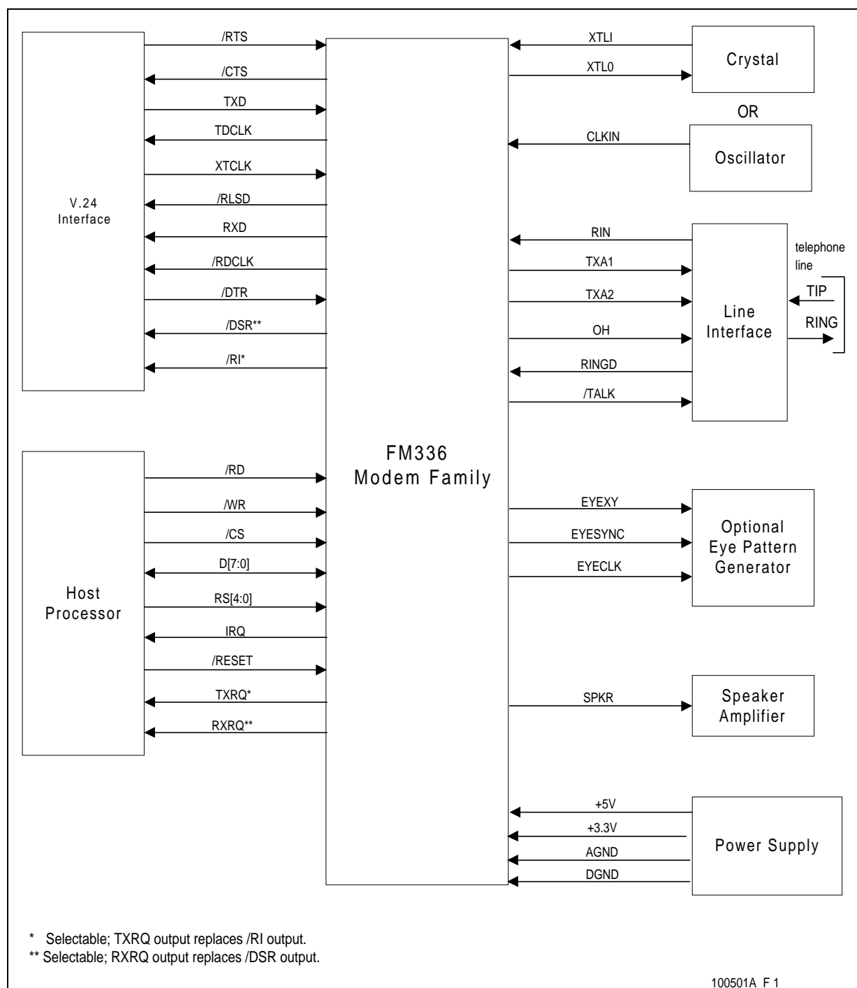
Figure 1. Functional Interface Signals
