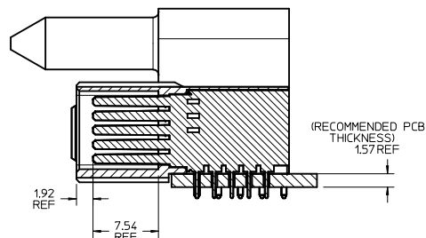
SECTION Z-Z
