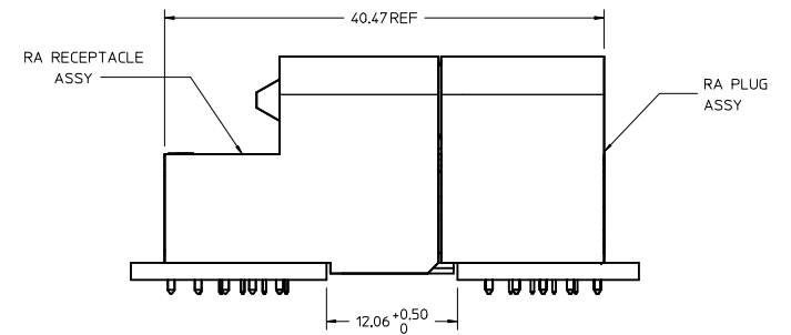
MATING PROFILE
