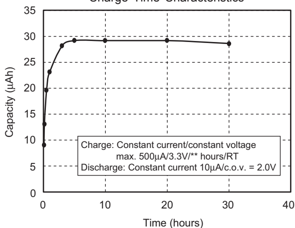
Charge Time Characteristics
