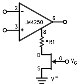
FET Current Sourcing Biasing
