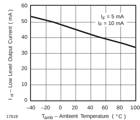
Figure 14. Low Level Output Current vs. Ambient Temperature
