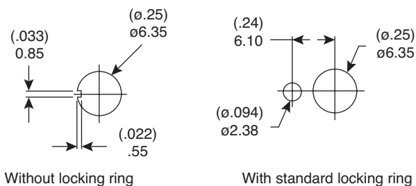
PANEL MOUNTING
