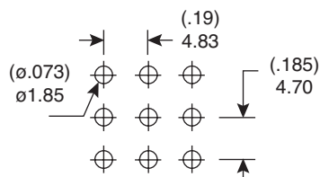
P.C. MOUNTING
