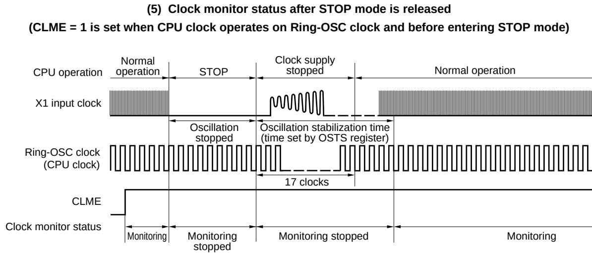
Figure 21-3. Timing of Clock Monitor (3/4)
