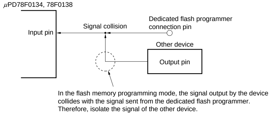
Figure 27-15. Signal Collision (Input Pin of Serial Interface)
