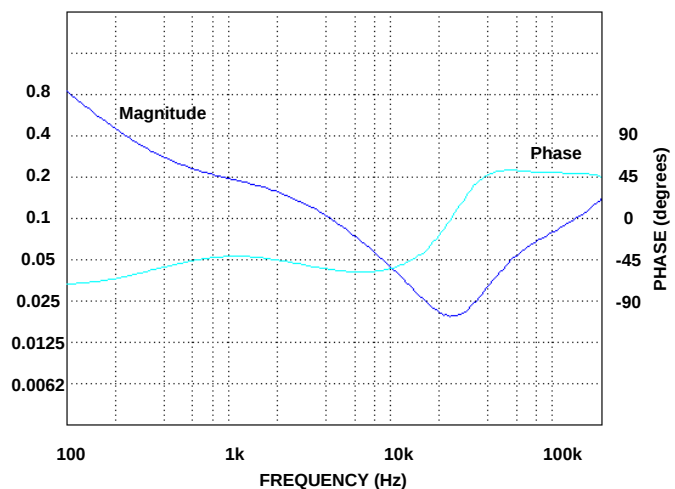
Model N6763A and N6765A, Option 760, CC Mode, @20 V, 15A
