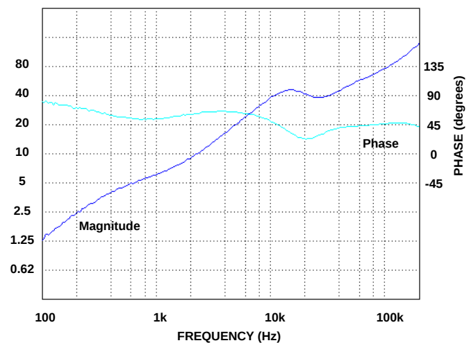
Model N6763A and N6765A, Option 760, CV Mode, @20 V, 15A
