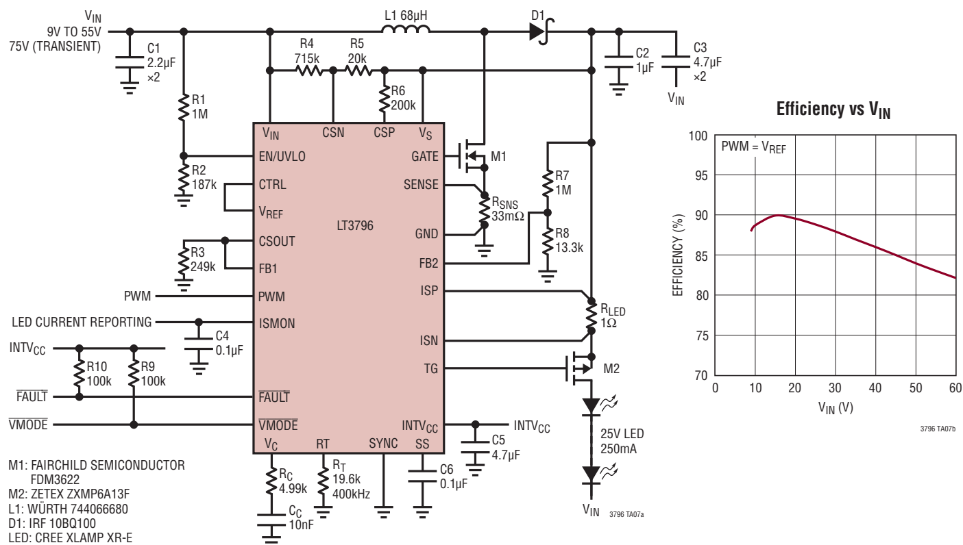
Buck-Boost Mode LED Driver with Open LED Clamp and Output Voltage Limit
