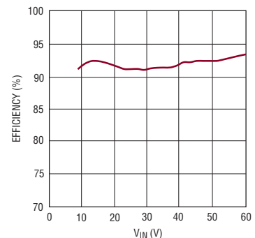
Efficiency vs V_{\text{IN}}
