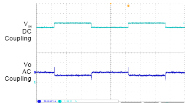
10. Line Transient
