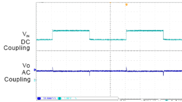
9. Line Transient
