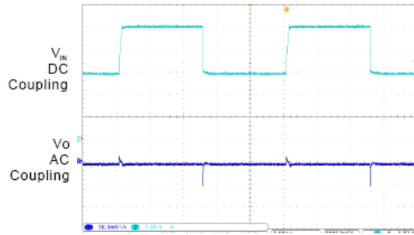
7. Line Transient
