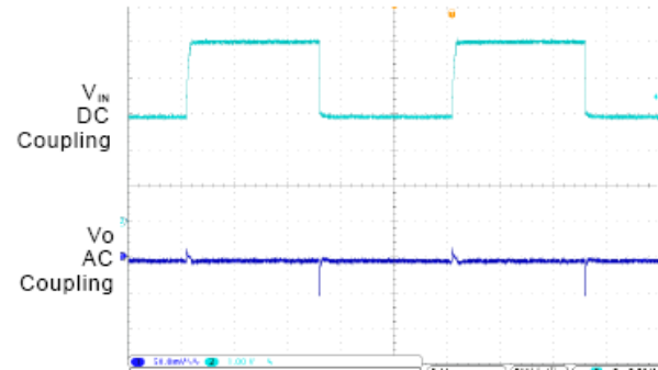
8. Line Transient
