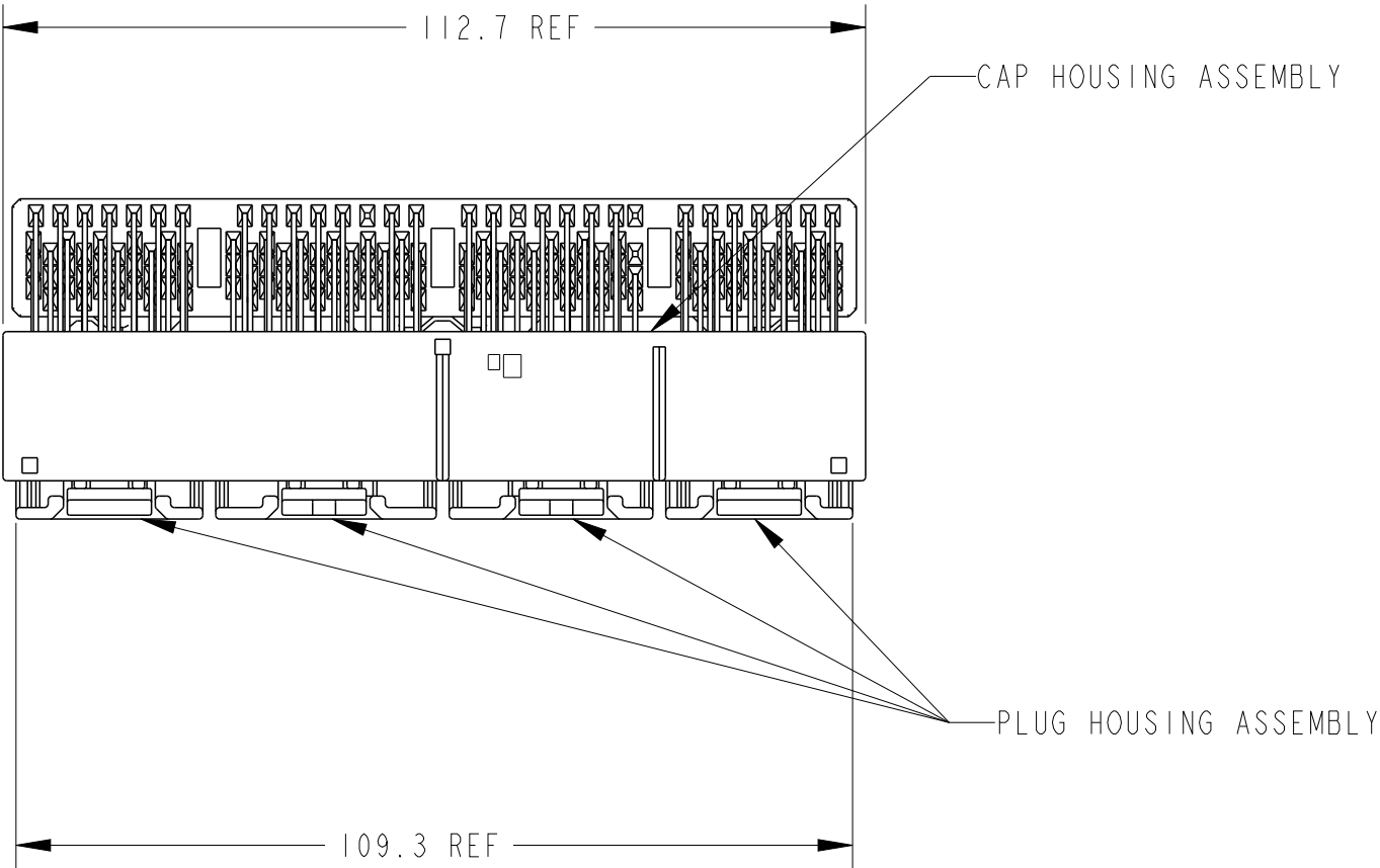
CAP HOUSING ASSEMBLY & PLUG HOUSING ASSEMBLY ENGAGEMENT VIEW CAP HOUSING ASSEMBLY & PLUG HOUSING ASSEMBLY 嵌合図
